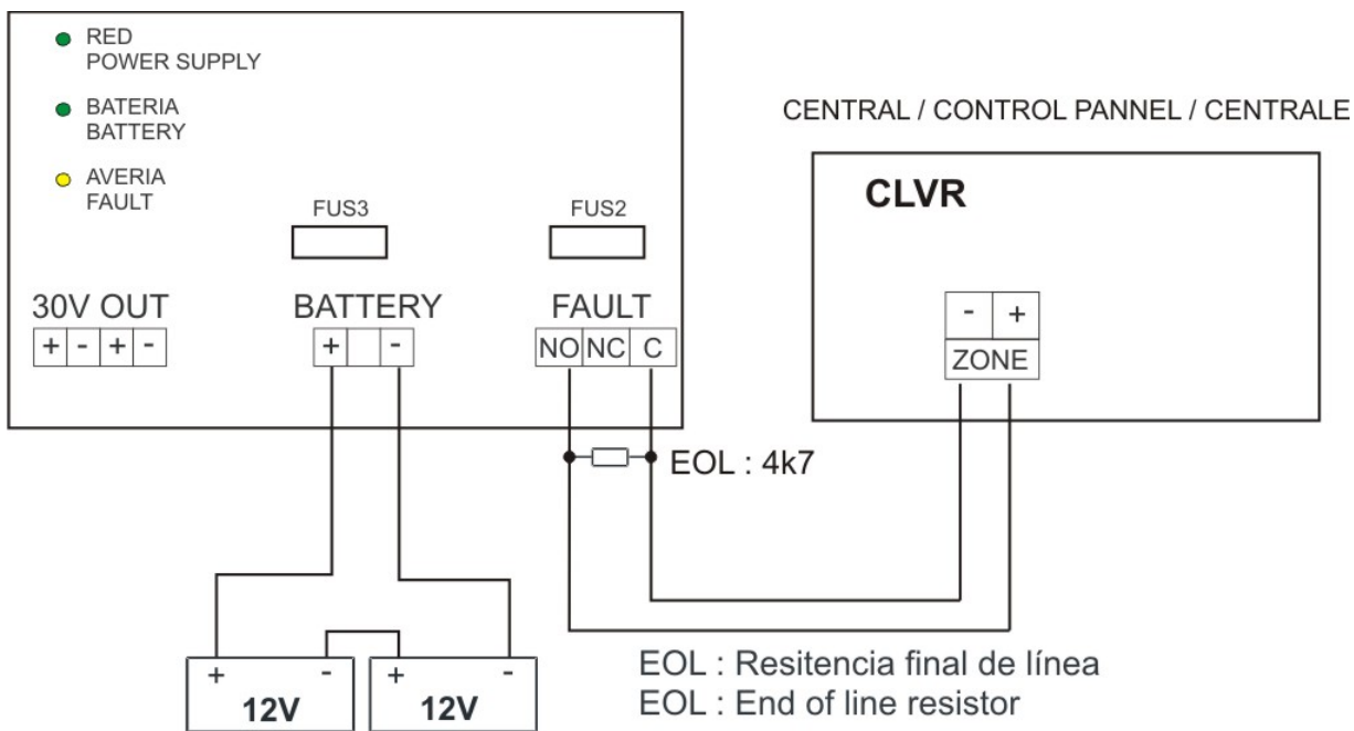
Figure 2: Fault output scheme
