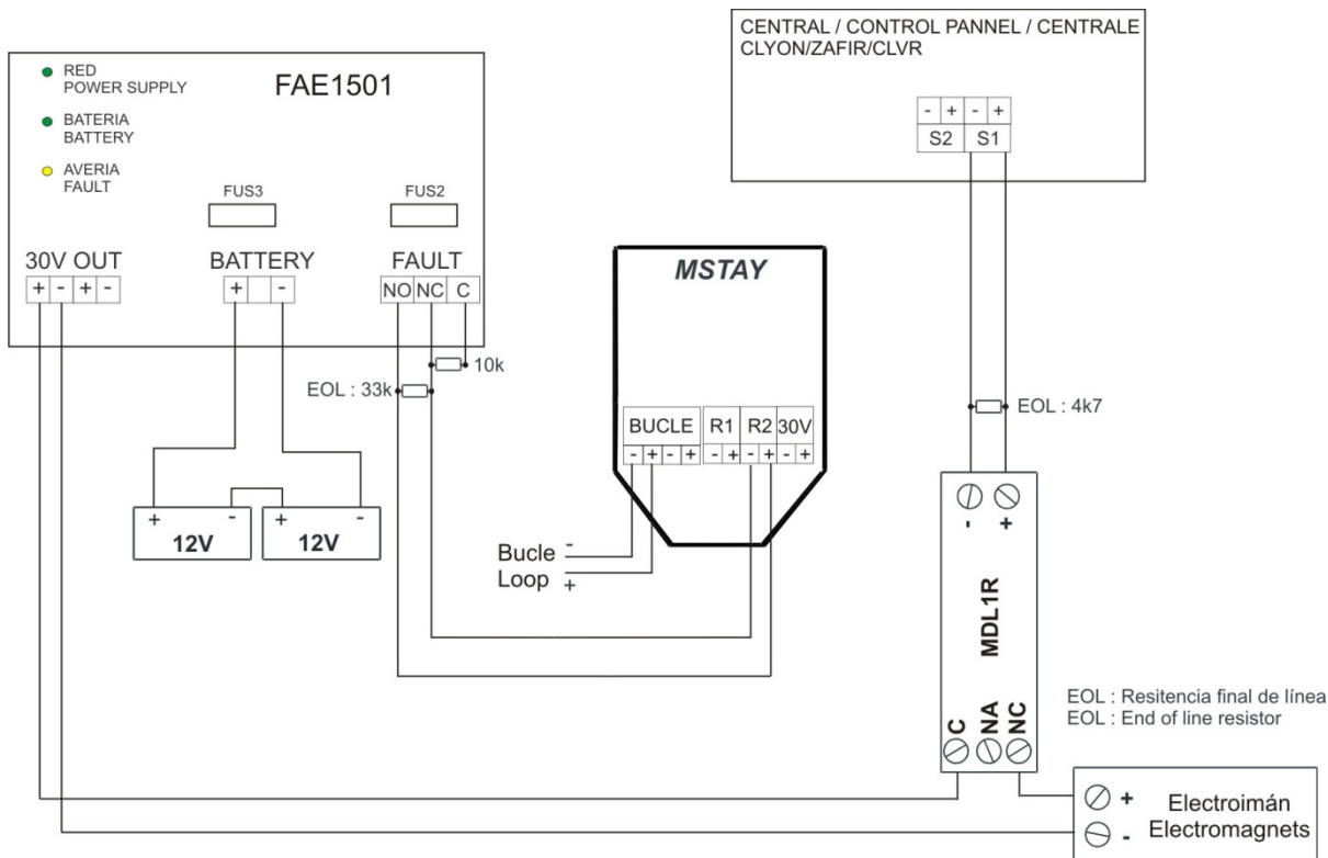
Figure 3: wiring diagram for addressable system and voltage free relay with electromagnet
